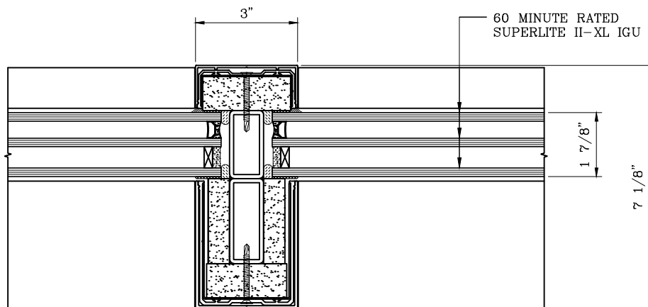
② VERTICAL MULLION DETAIL
