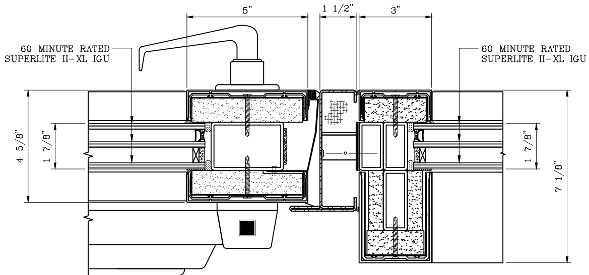
13 DOOR JAMB at LOCK DETAIL
