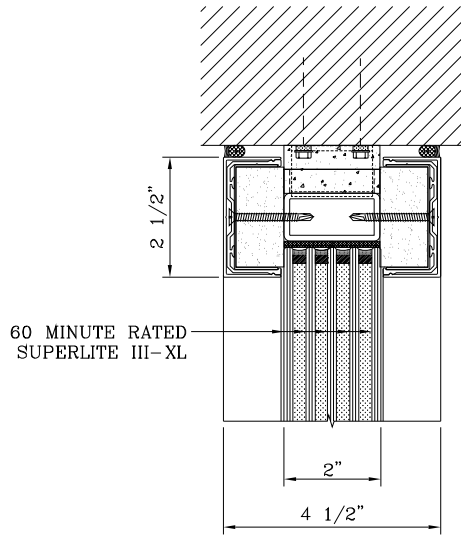
4 HEAD DETAIL
