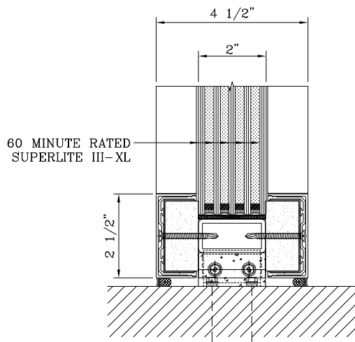
5 SILL DETAIL
