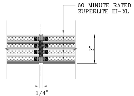
14 BUTT-GLAZED DETAIL
