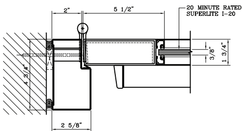
Door Jamb at Hinge Detail
