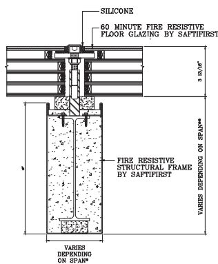
2 BEAM DETAIL
