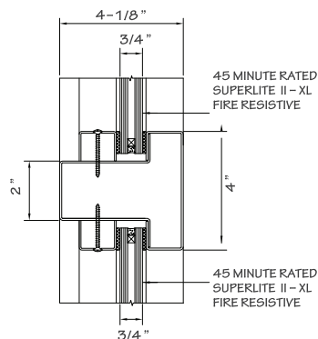
Horizontal Mullion
