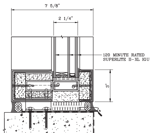
Sill Detail
