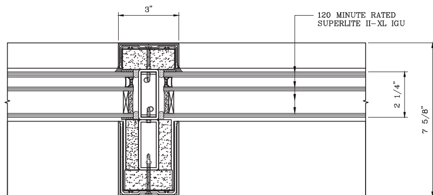
Vertical Mullion
