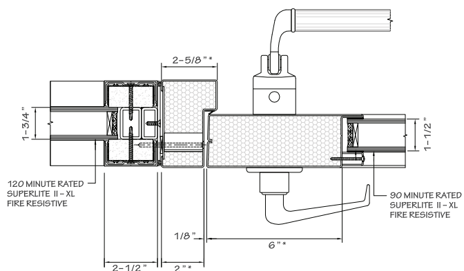
Shown in standard profile with glazed-in stop
