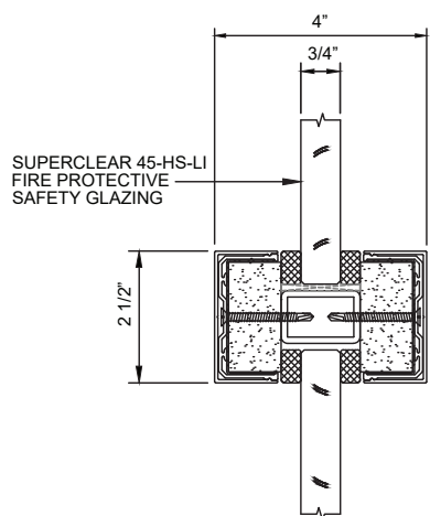
HORIZONTAL MULLION DETAIL
