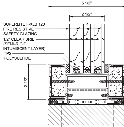
SILL DETAIL
