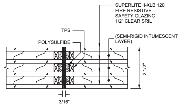
BUTT-GLAZED DETAIL
