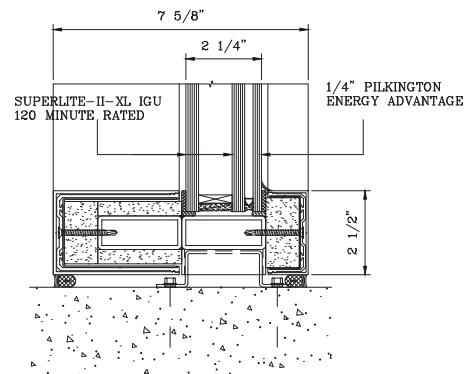
SILL DETAIL
