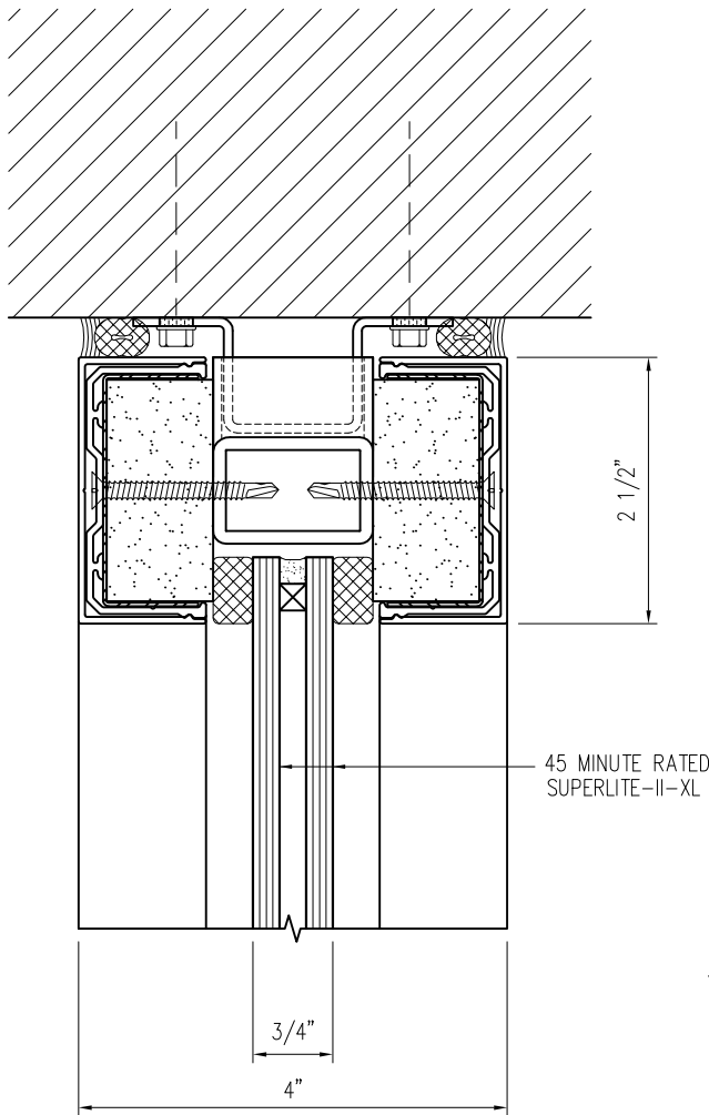
38a HEAD DETAIL 60 GPX-0-45R-IIXL
