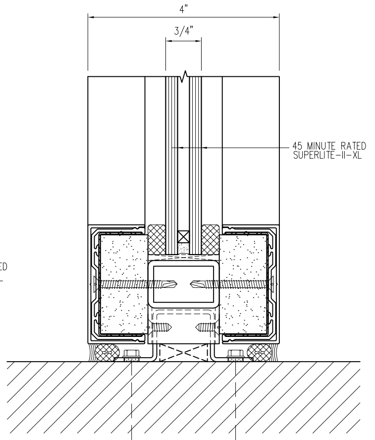
41a SILL DETAIL 60 GPX-0-45R-IIXL
