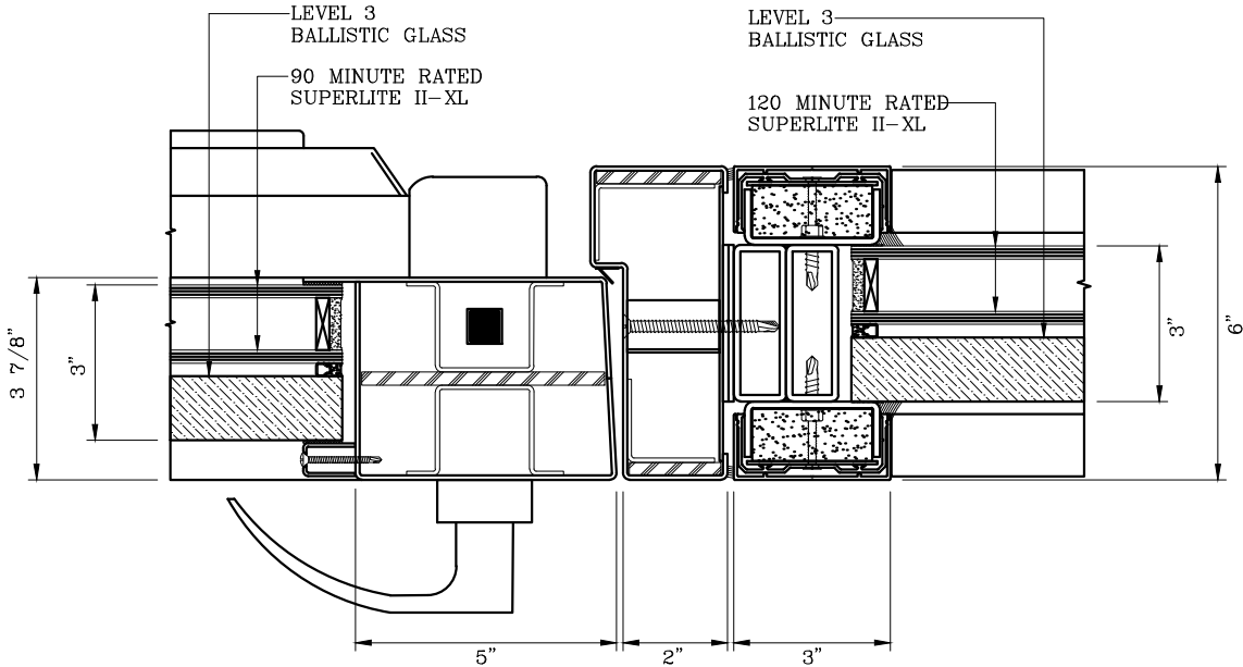
9 DOOR MEETING STILES DETAIL
