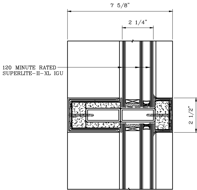
3 HORIZONTAL MULLION DETAIL
