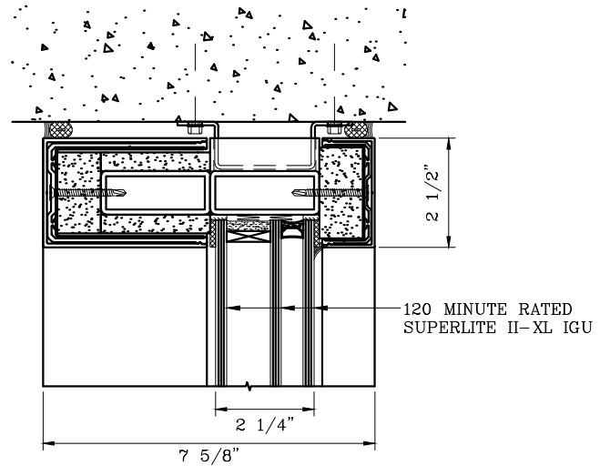
4 HEAD DETAIL
