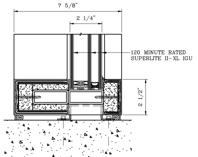
5 SILL DETAIL
