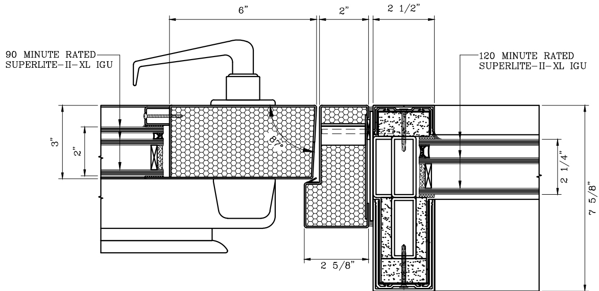
9 DOOR MEETING STILES DETAIL
