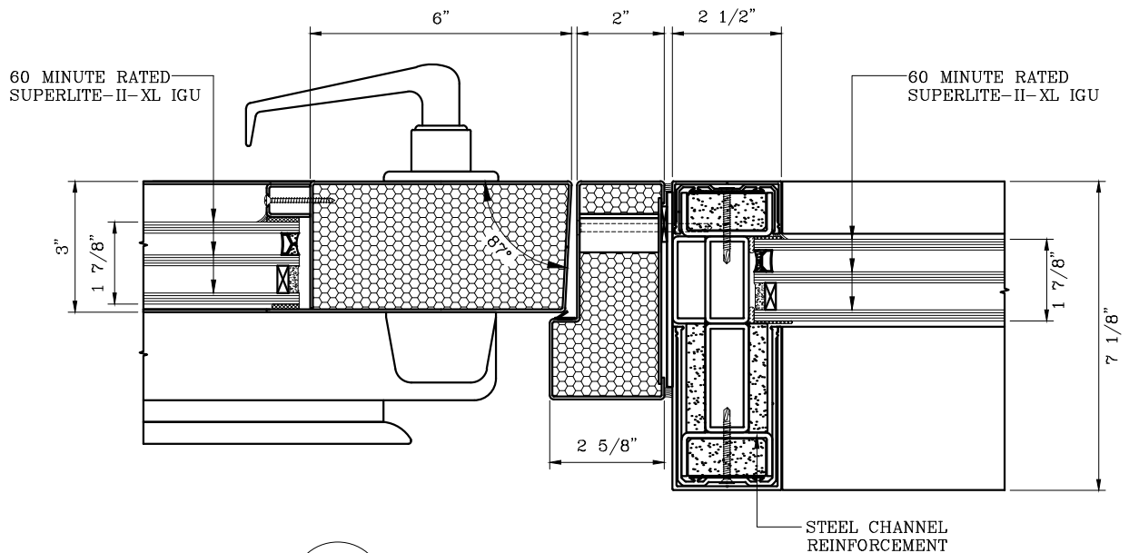
9 DOOR MEETING STILES DETAIL
