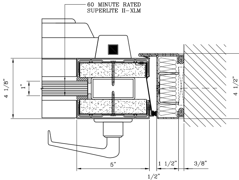
12 DOOR JAMB at LOCK
