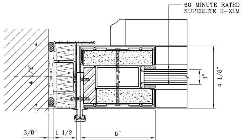
11 DOOR JAMB at HINGE
