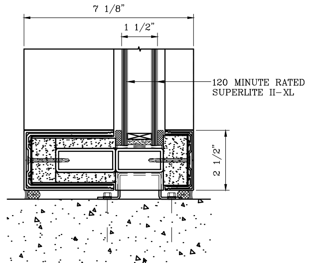
5 SILL DETAIL
