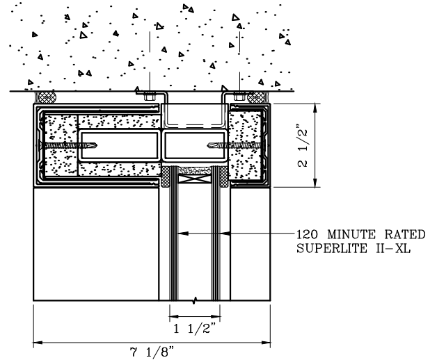
4 HEAD DETAIL
