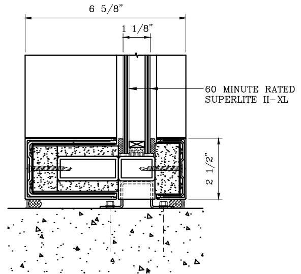
5 SILL DETAIL
