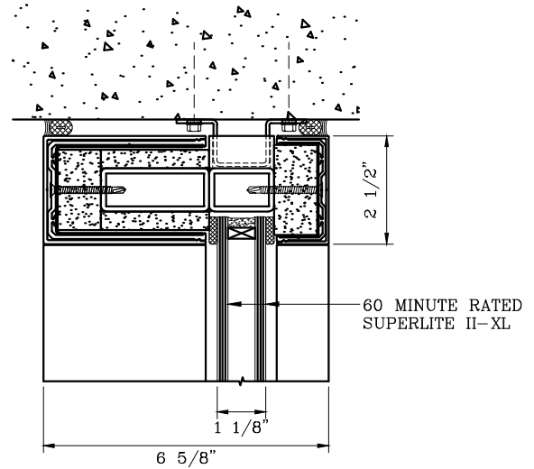
4 HEAD DETAIL
