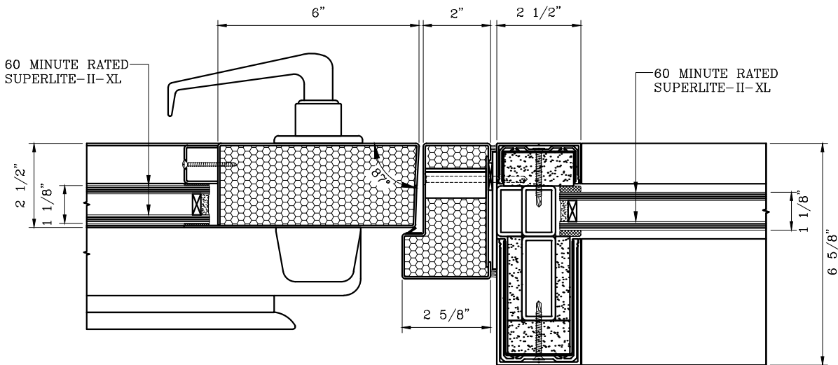
9 DOOR JAMB at LOCK DETAIL
