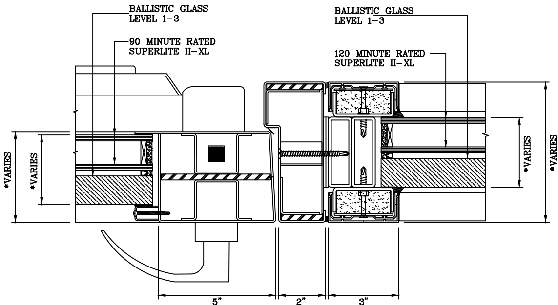
9 DOOR MEETING STILES DETAIL
