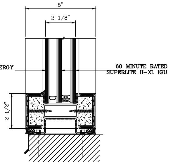
5 SILL DETAIL
