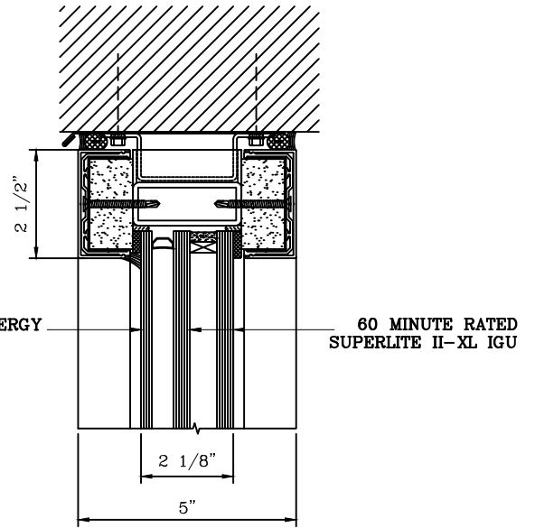
4 HEAD DETAIL
