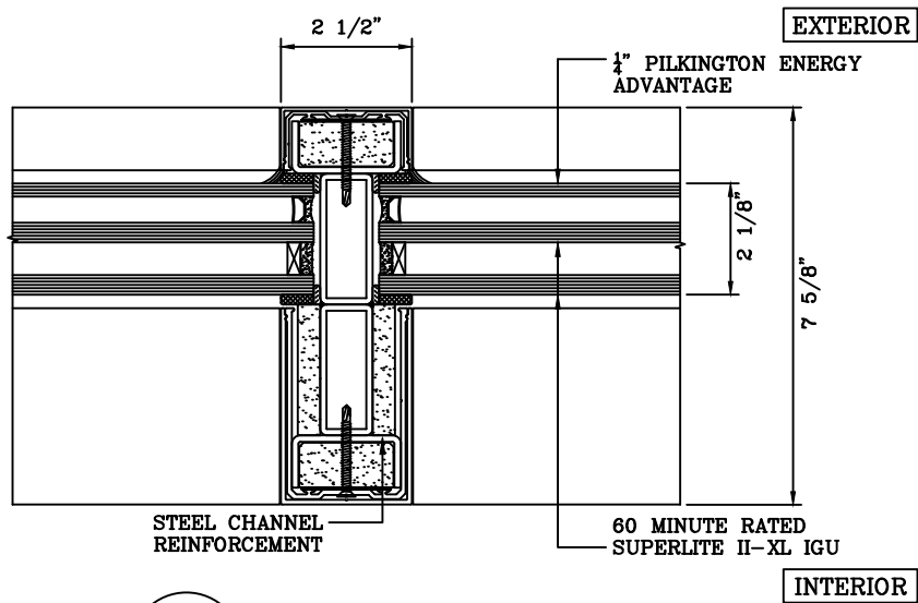
2 VERTICAL MULLION DETAIL
