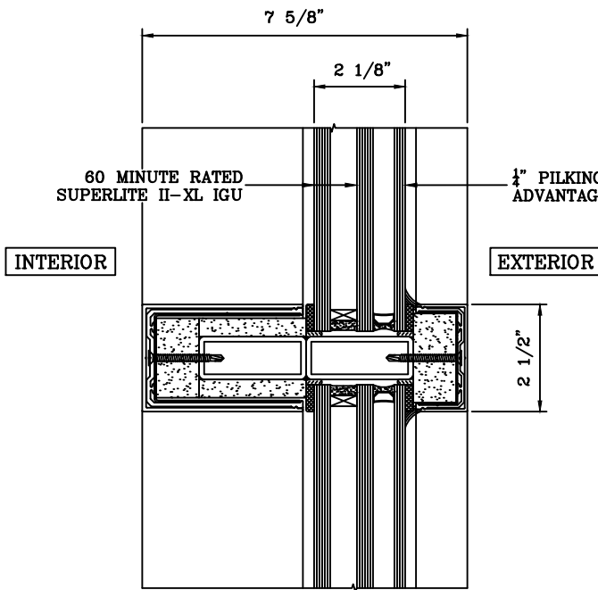
3 HORIZONTAL MULLION DETAIL
