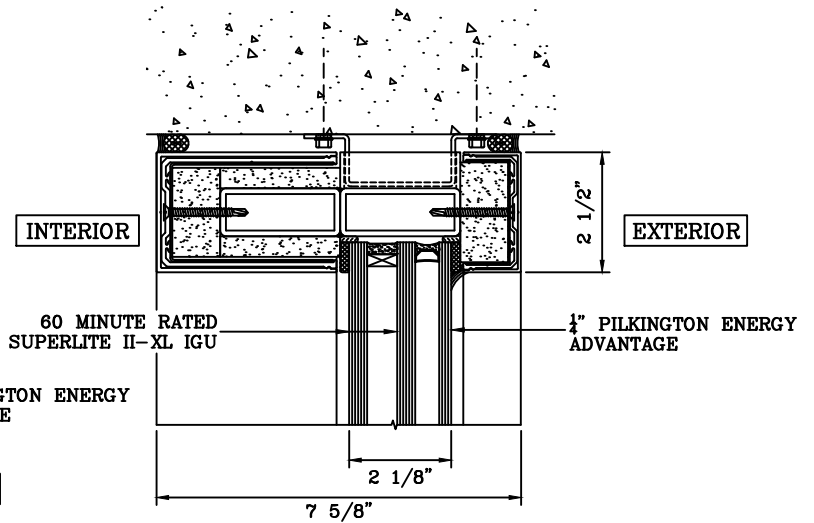
4 HEAD DETAIL
