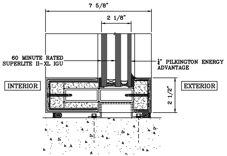
5 SILL DETAIL
