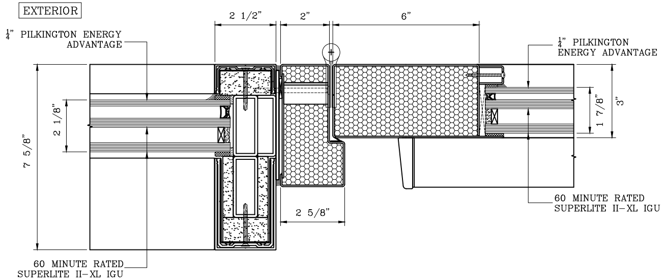
8 DOOR JAMB at HINGE DETAIL
