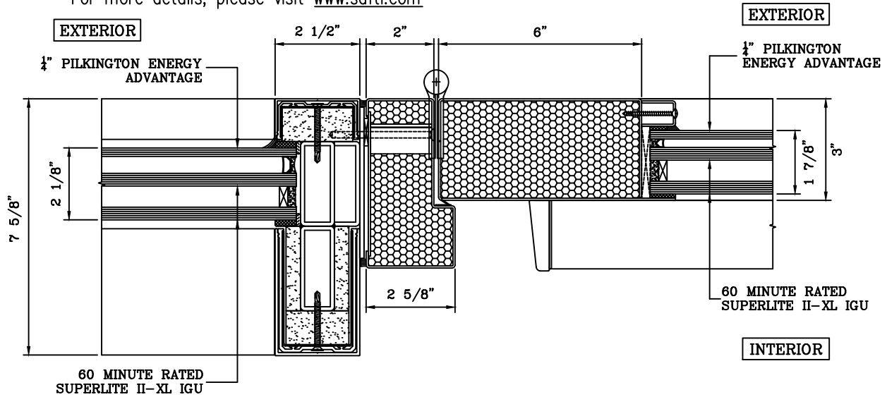
DOOR JAMB at HINGE DETAIL
