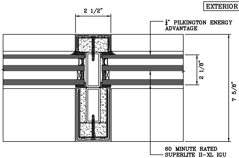
2 VERTICAL MULLION DETAIL EXTERIOR
