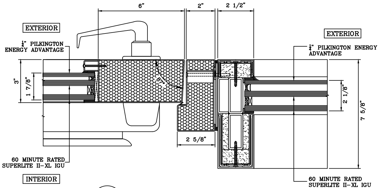
DOOR MEETING STILES DETAIL
