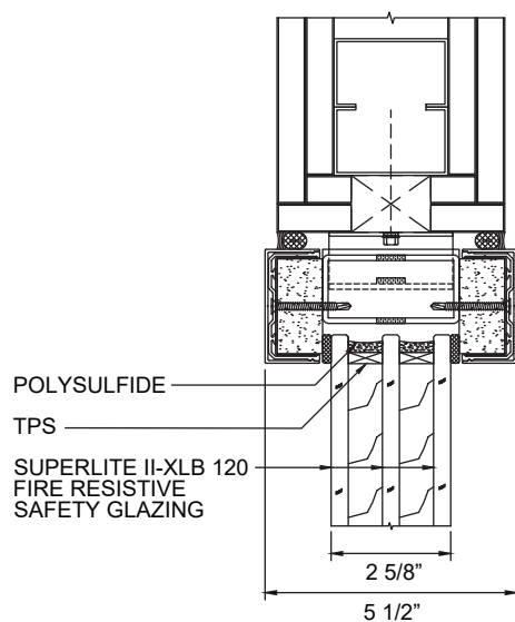
HEAD DETAIL
