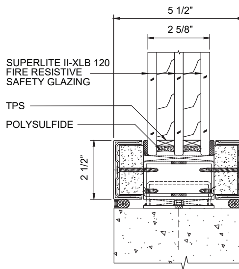
SILL DETAIL
