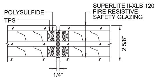
BUTT-GLAZED DETAIL
