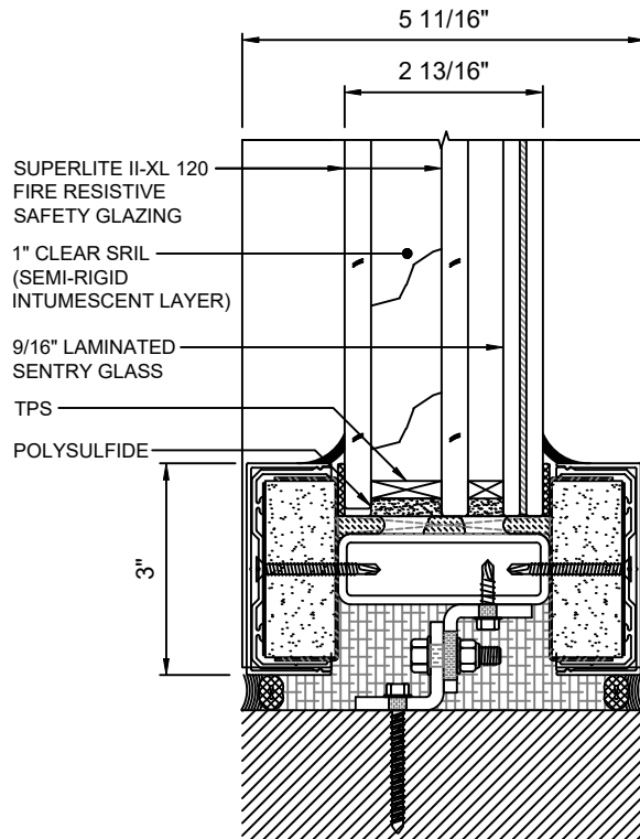
A SILL DETAIL 5 WITH SUPERLITE II-XL 120
