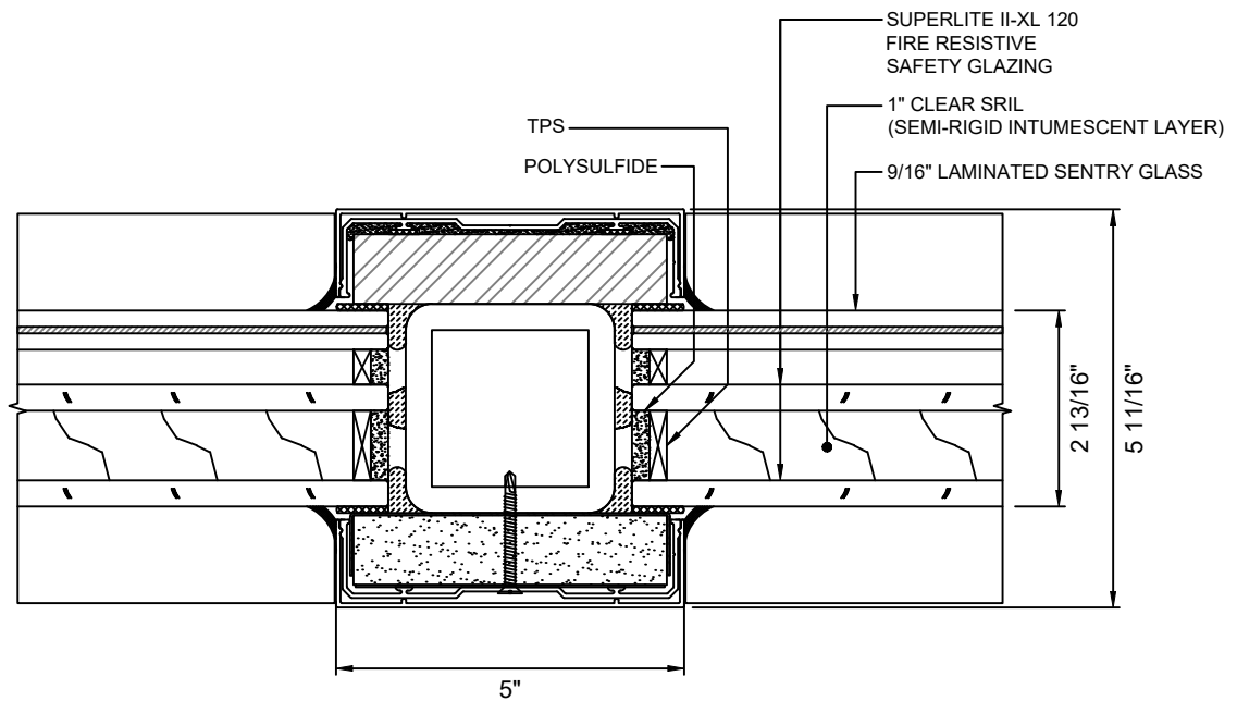
(A) 7 VERTICAL MULLION DETAIL WITH SUPERLITE II-XL 120
