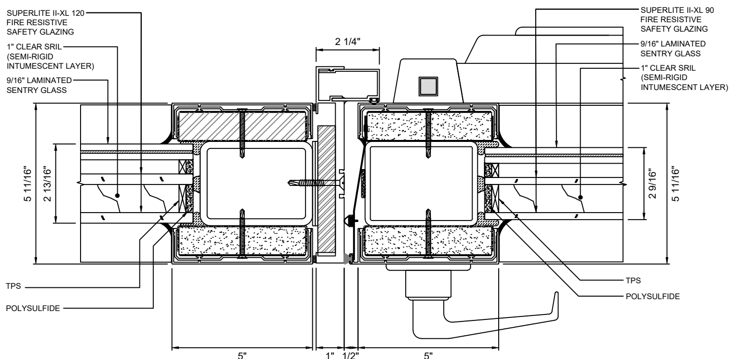
(A) 10 DOOR JAMB AT LOCK WITH SUPERLITE II-XL 90 & II-XL 120
