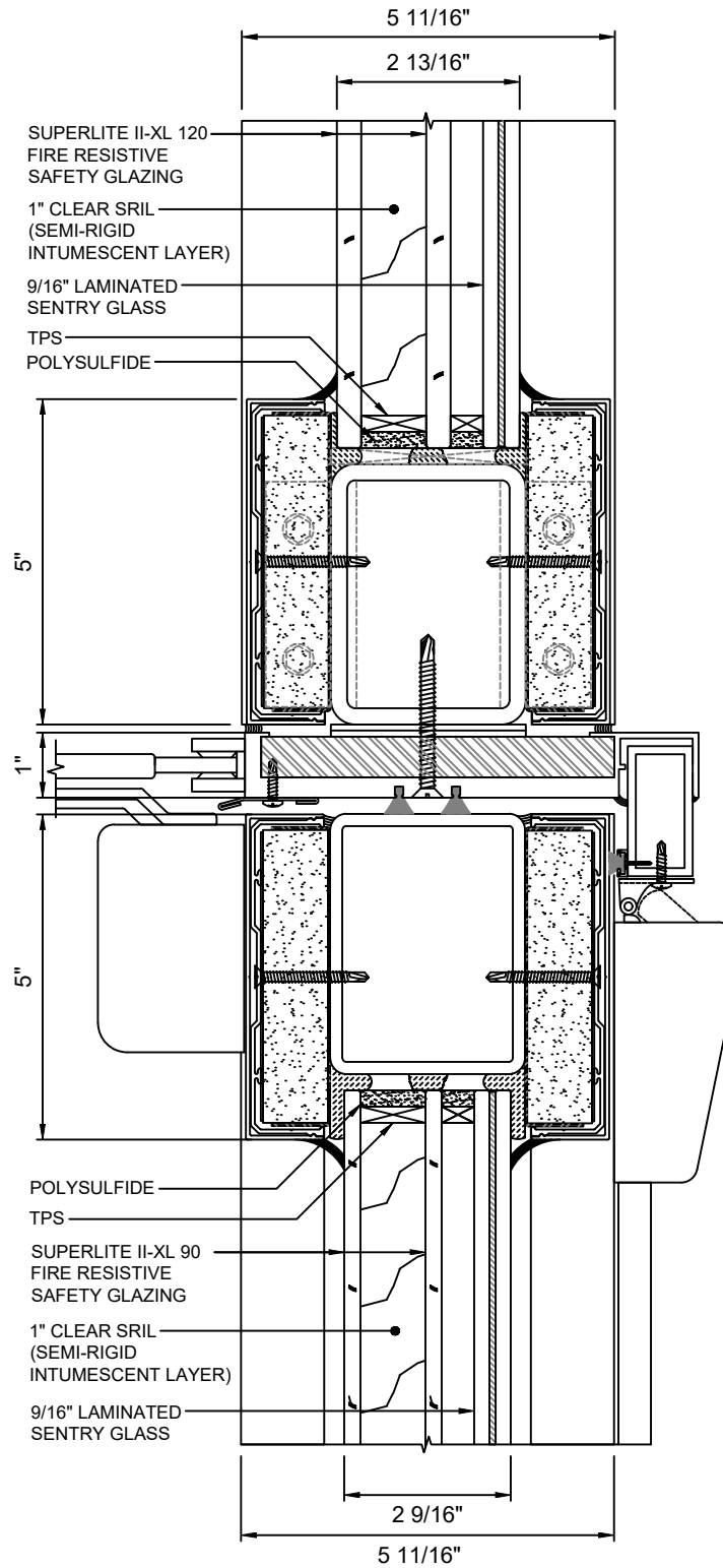
A 8 DOOR TOP RAIL WITH SUPERLITE II-XL 90 & II-XL 120
