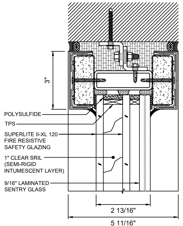
A HEAD DETAIL 3 WITH SUPERLITE II-XL 120
