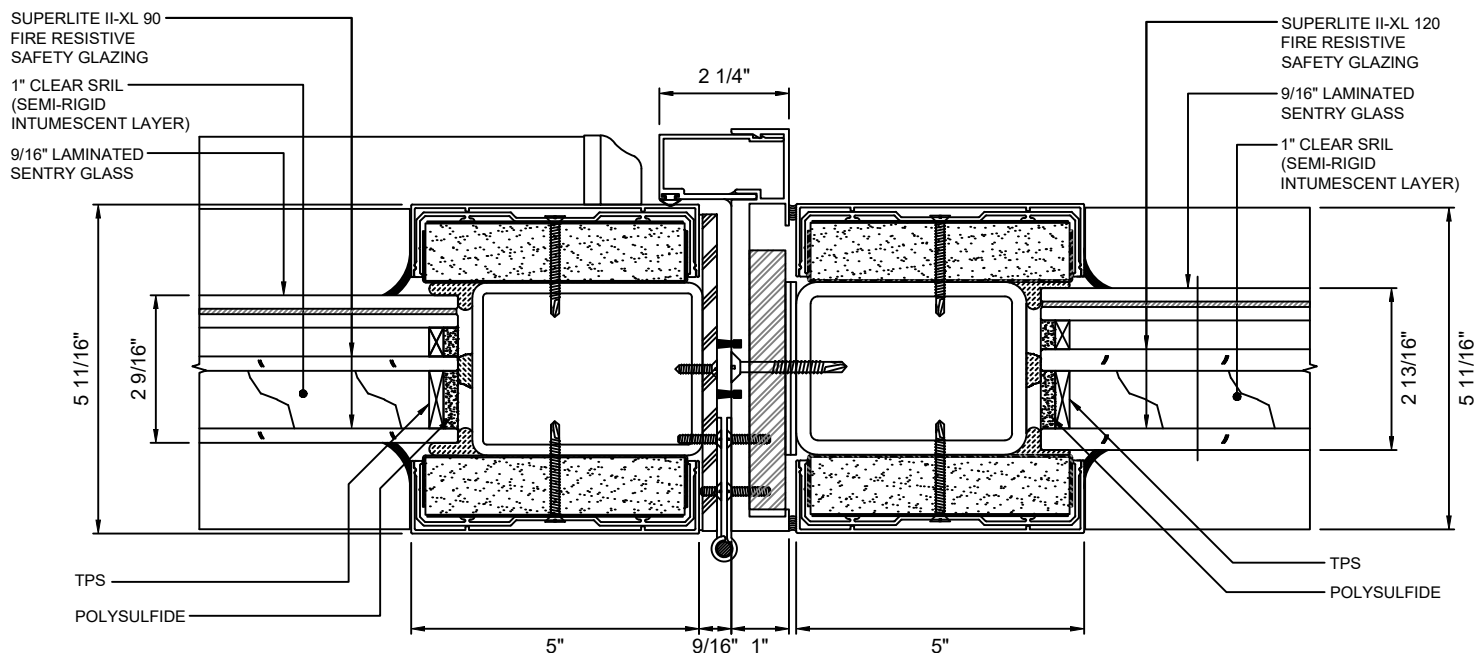
A 11 DOOR JAMB AT HINGE WITH SUPERLITE II-XL 90 & II-XL 120
