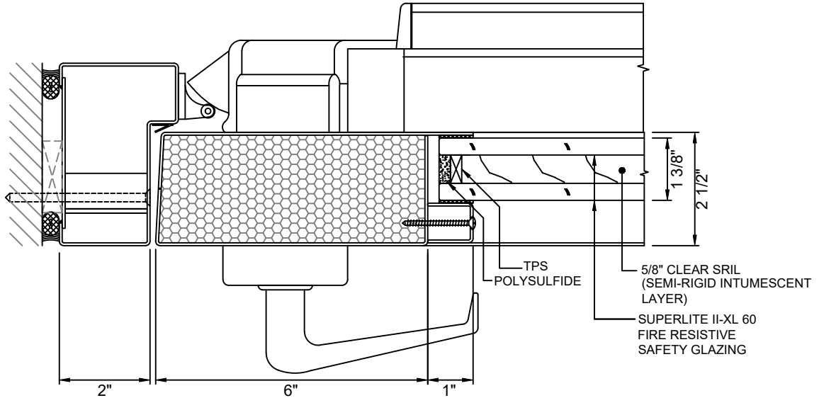
(A) 4 DOOR JAMB AT LOCK - STANDARD WITH SUPERLITE II-XL 60
