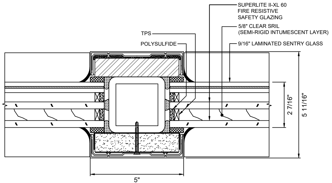
Ⓐ 7 VERTICAL MULLION DETAIL WITH SUPERLITE II-XL 60
