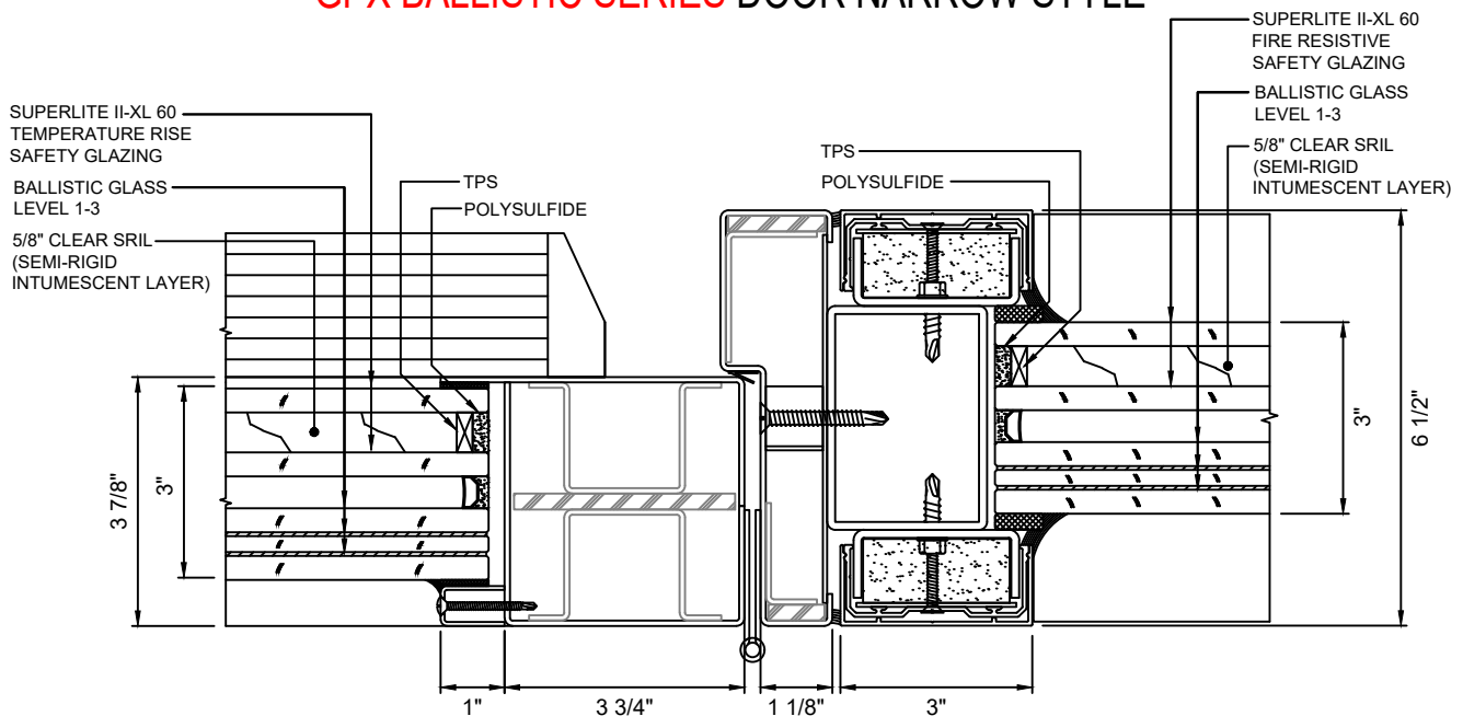
(G) DOOR JAMB AT HINGE - NARROW STYLE 16 WITH SUPERLITE II-XL 60 WITH LEVEL 1-3 BALLISTIC GLASS
