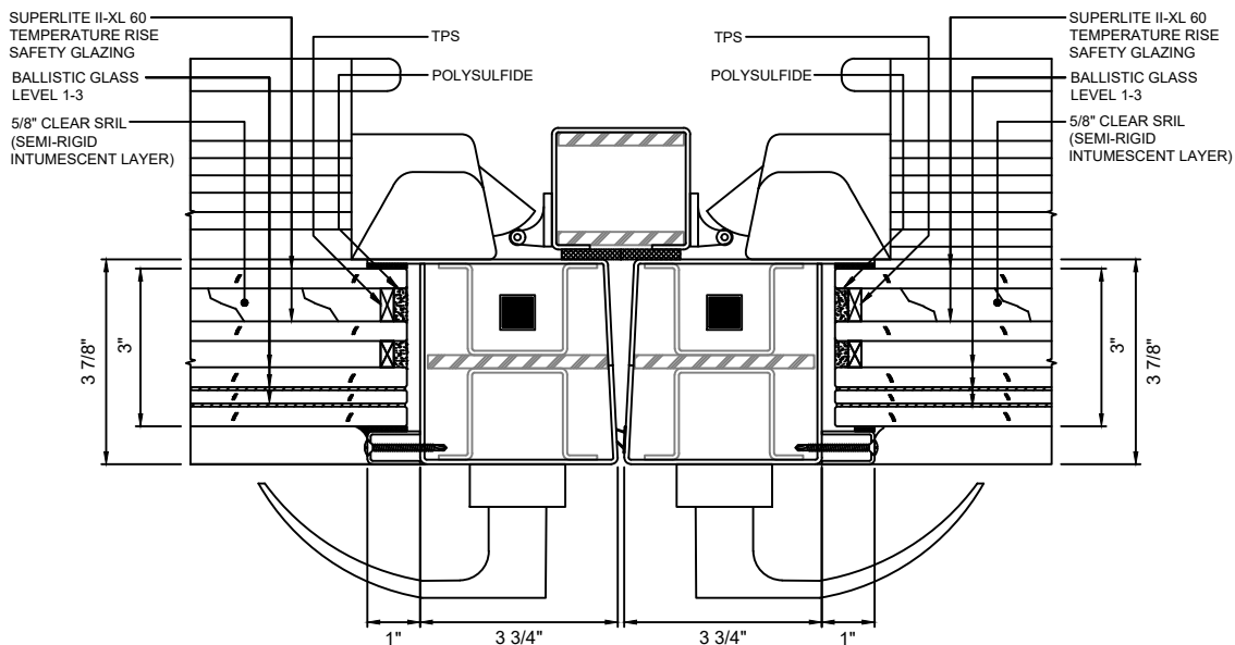
G 17 MEETING STILES - NARROW STYLE WITH SUPERLITE II-XL 60 WITH LEVEL 1-3 BALLISTIC GLASS
