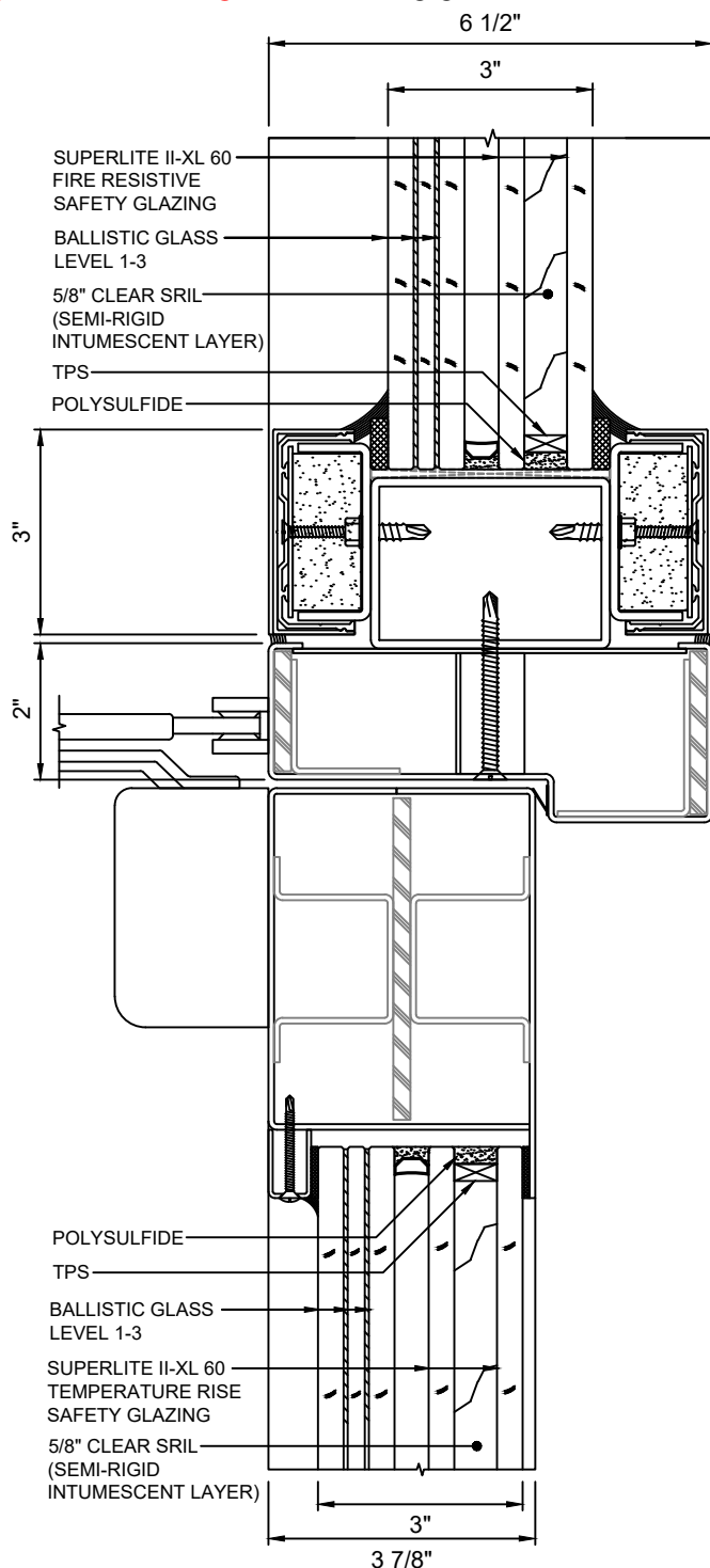
F 13 DOOR TOP RAIL - STANDARD WITH SUPERLITE II-XL 60 WITH LEVEL 1-3 BALLISTIC
