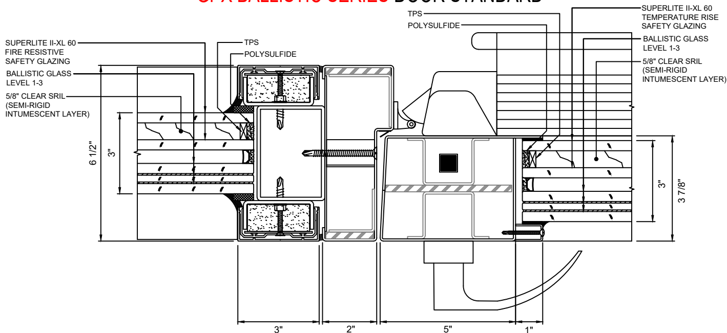
F 15 DOOR JAMB AT LOCK - STANDARD WITH SUPERLITE II-XL 60 WITH LEVEL 1-3 BALLISTIC GLASS
