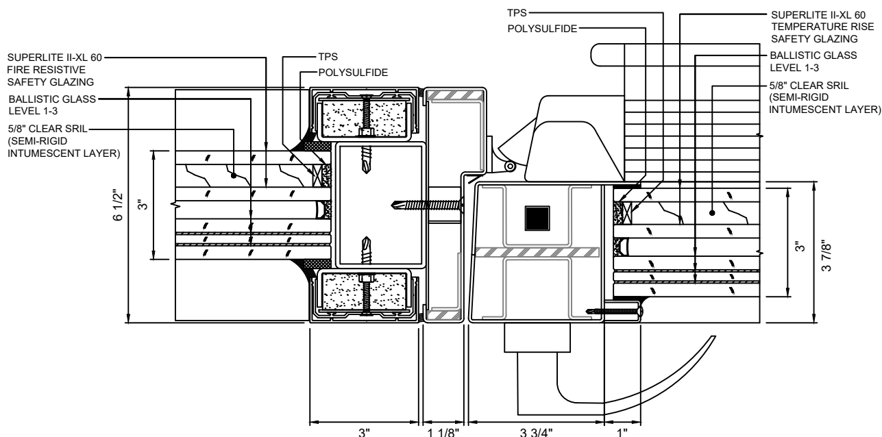
G 15 DOOR JAMB AT LOCK - NARROW STYLE WITH SUPERLITE II-XL 60 WITH LEVEL 1-3 BALLISTIC GLASS
