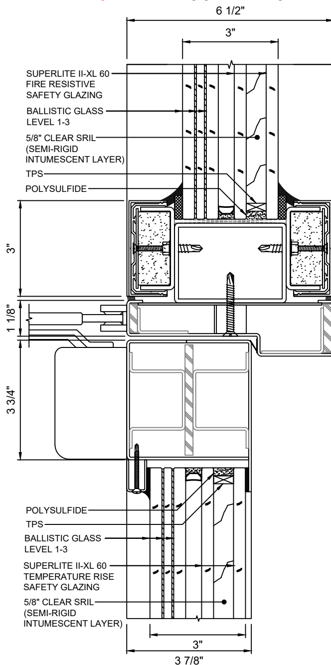
G 13 DOOR TOP RAIL - NARROW STYLE WITH SUPERLITE II-XL 60 WITH LEVEL 1-3 BALLISTIC GLASS
