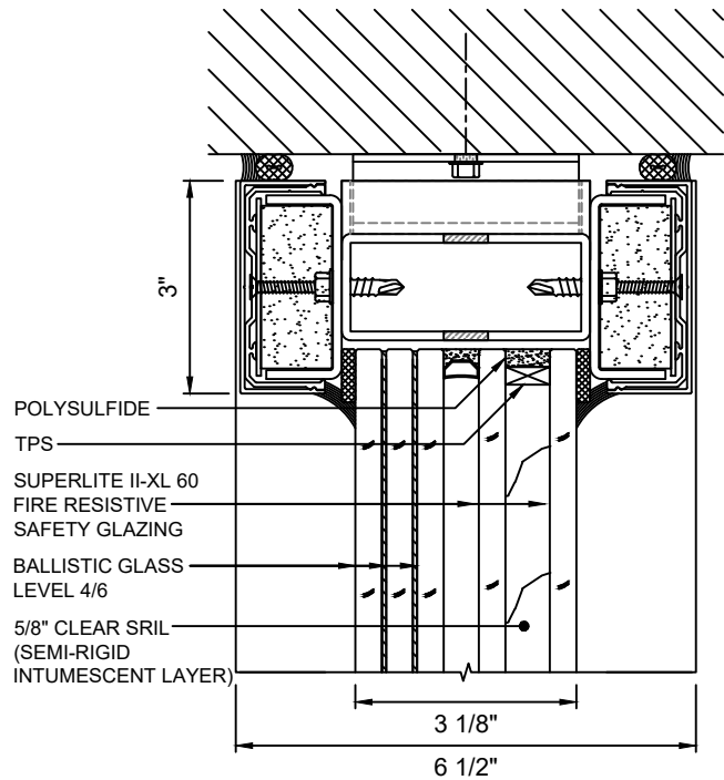
B 3 HEAD DETAIL WITH SUPERLITE II-XL 60 WITH LEVEL 4/6 BALLISTIC GLASS
