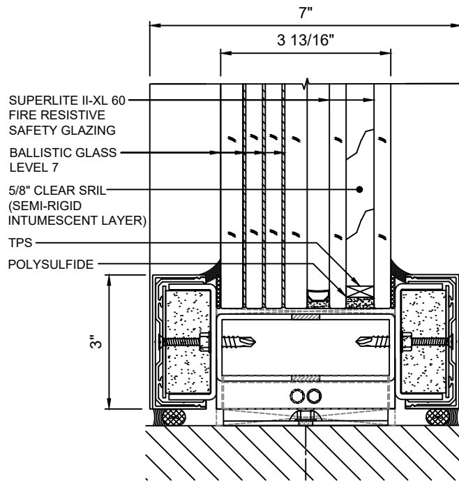
D 8 SILL DETAIL WITH SUPERLITE II-XL 60 WITH LEVEL 7 BALLISTIC GLASS
