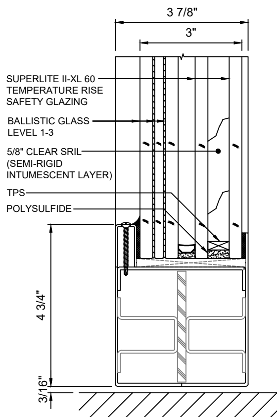
G 14 DOOR BOTTOM RAIL - NARROW WITH SUPERLITE II-XL 60 WITH LEVEL 1-3 BALLISTIC GLASS
