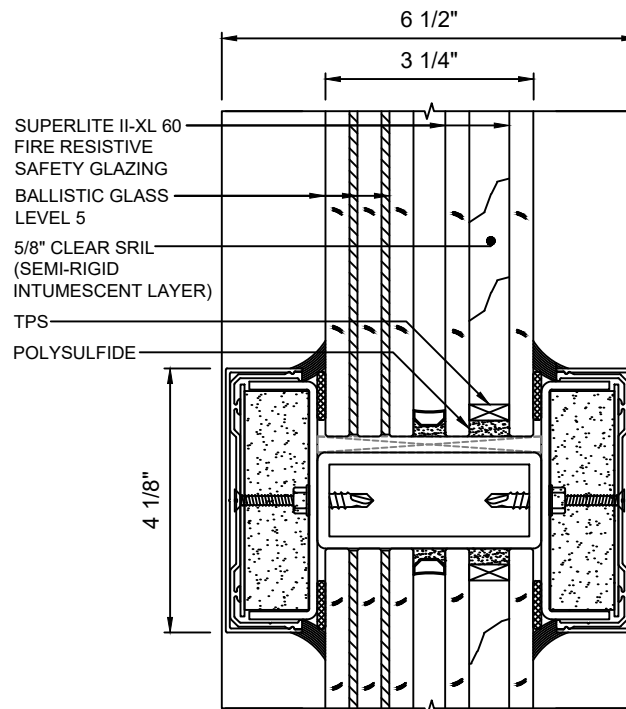
C 5 HORIZONTAL MULLION WITH SUPERLITE II-XL 60 WITH LEVEL 5 BALLISTIC GLASS
