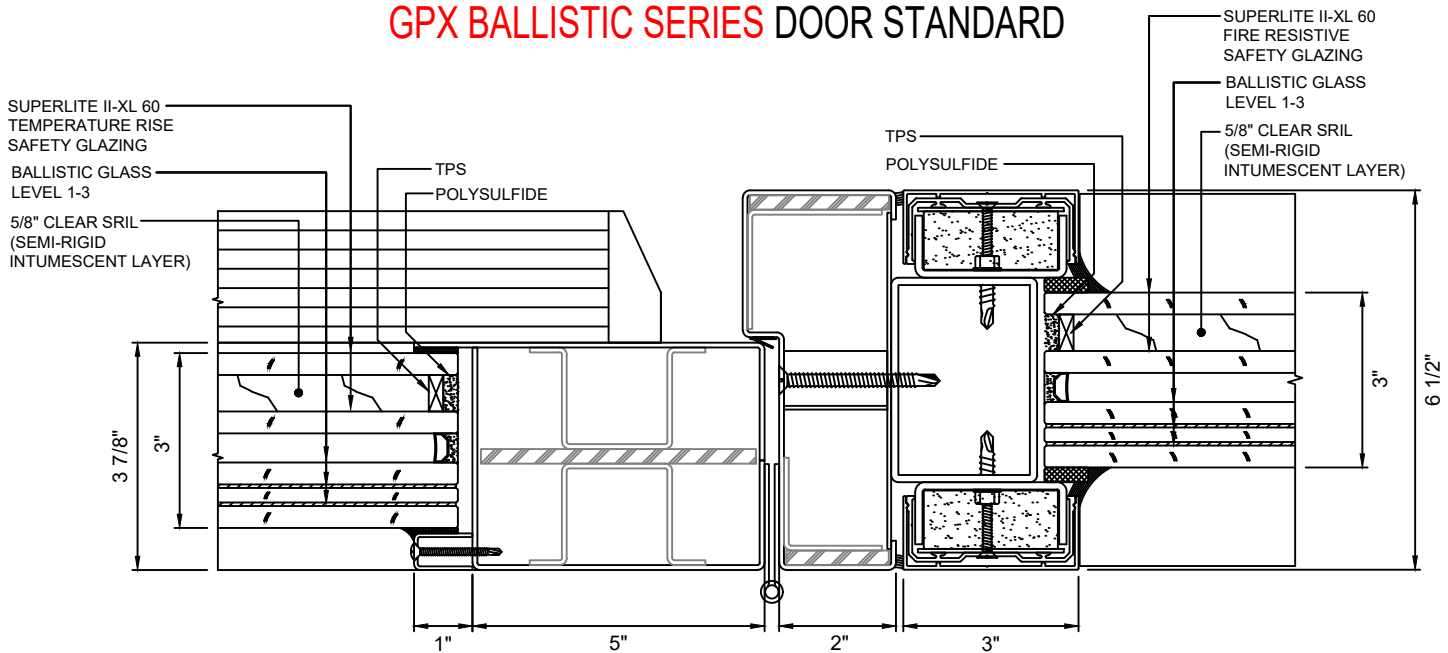
(F) DOOR JAMB AT HINGE - STANDARD 16 WITH SUPERLITE II-XL 60 WITH LEVEL 1-3 BALLISTIC GLASS
