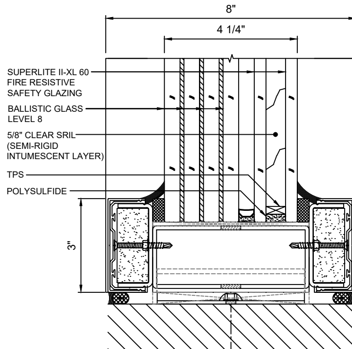
E 8 SILL DETAIL WITH SUPERLITE II-XL 60 WITH LEVEL 8 BALLISTIC GLASS
