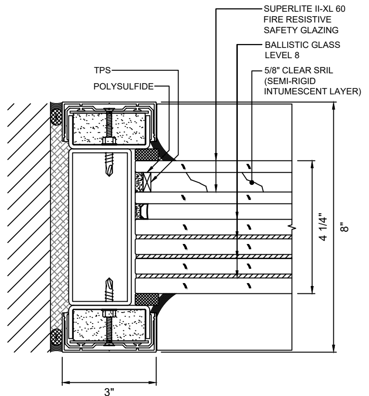
E 10 JAMB DETAIL WITH SUPERLITE II-XL 60 WITH LEVEL 8 BALLISTIC GLASS
