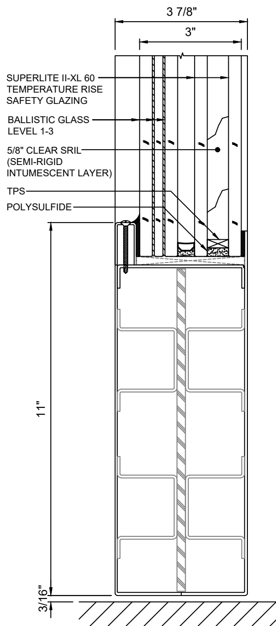
F 14 DOOR BOTTOM RAIL - STANDARD WITH SUPERLITE II-XL 60 WITH LEVEL 1-3 BALLISTIC GLASS
