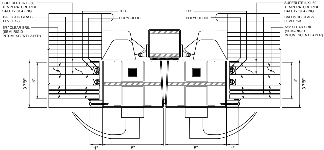
F 17 MEETING STILES - STANDARD WITH SUPERLITE II-XL 60 WITH LEVEL 1-3 BALLISTIC GLASS
